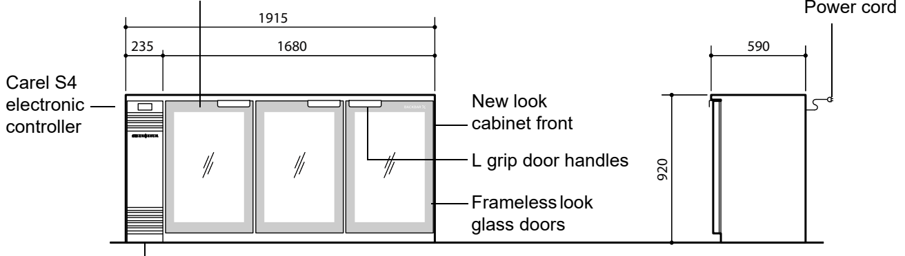
Side mounted remote refrigeration unit
